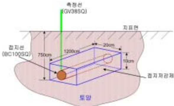
(그림2-9) 접지저감제의 설계 구조 Figure 2.5 Design Structure of Grounding Resistance Enhancement Materials
