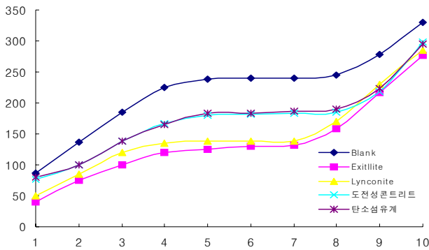
그림2-14. 접지저감제별 접지저항 측정치 Figure 2.14. The kinds of grounding resistance lawing agents for grounding resistance result
